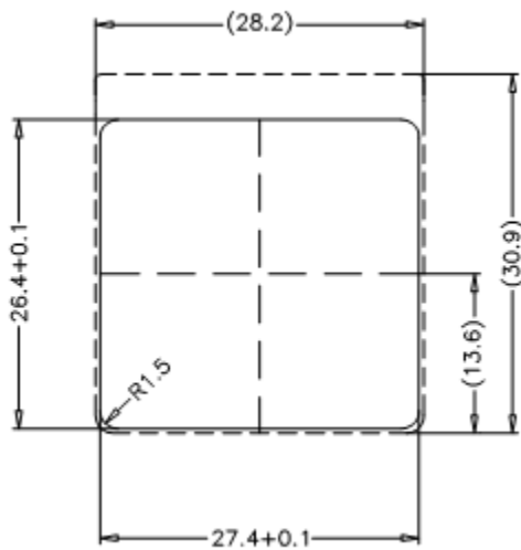
Panel Cutout
